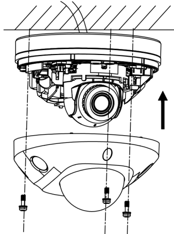
Figure 2-21 Installing Front Cover
