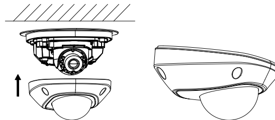
Figure 2-12 Installing Front Cover
