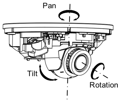
Figure 2-20 Adjusting Angle
