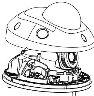
Figure 2-15 Removing Front Cover
