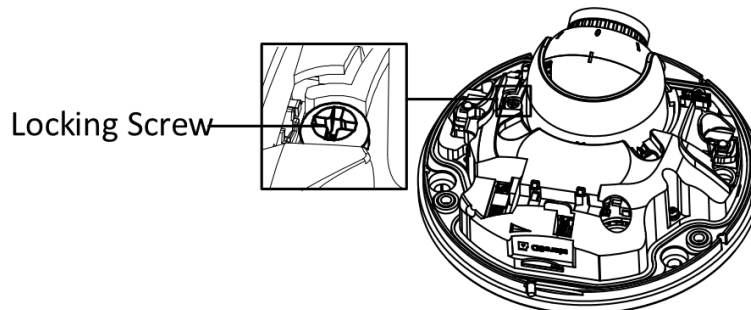
Figure 2-19 Loosen Locking Screw
