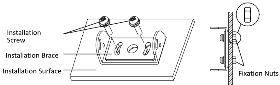
Figure 2-26 Installing Support
