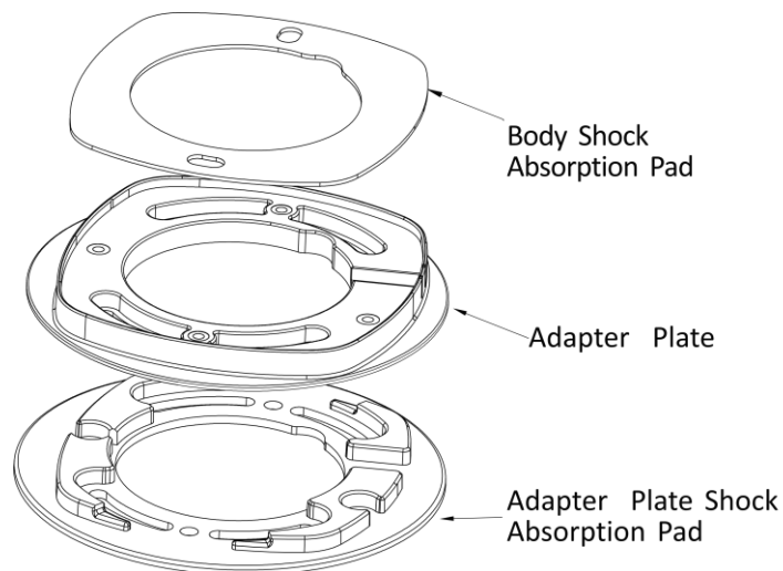
Figure 2-5 Shock Absorption Pads and Adapter
