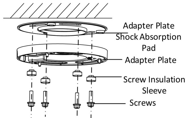
Figure 2-17 Install Adapter Plate
