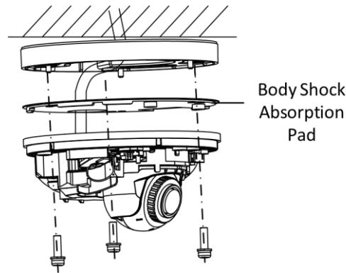
Figure 2-18 Fasten Base
