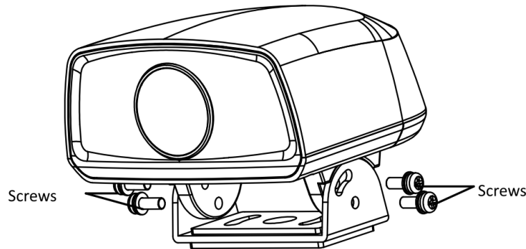
Figure 2-24 Removing Camera Bracket
