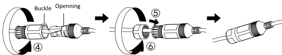
Figure 5-3 Complete Installation
