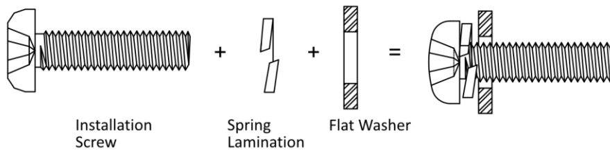
Figure 2-25 Assemble Screws
