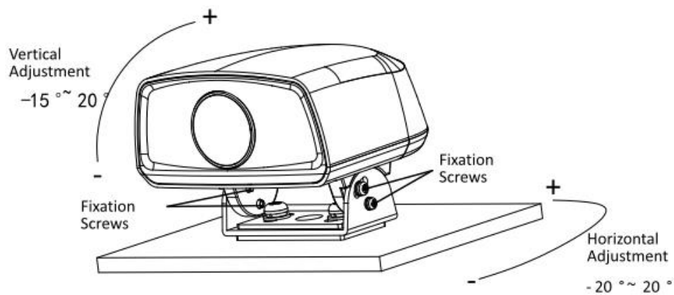
Figure 2-28 Adjusting Angle
