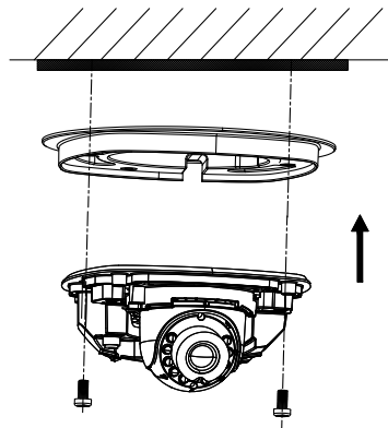
Figure 2-10 Fixed Base
