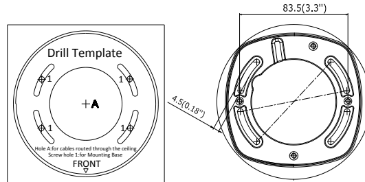
Figure 2-4 Drill Templates and Adapter Plate
