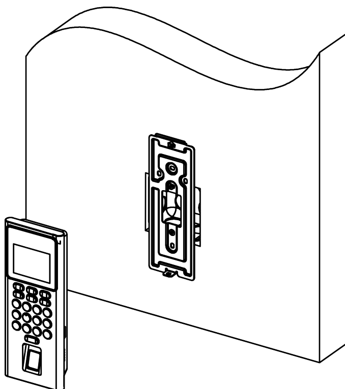
Figure 2-3 Secure Device
