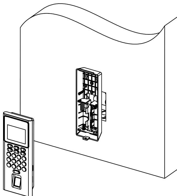
Figure 2-6 Hang Device
