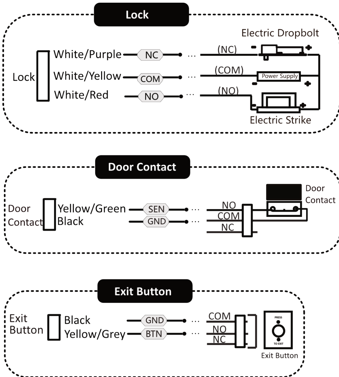
Figure 3-1 Wiring Terminal Description
