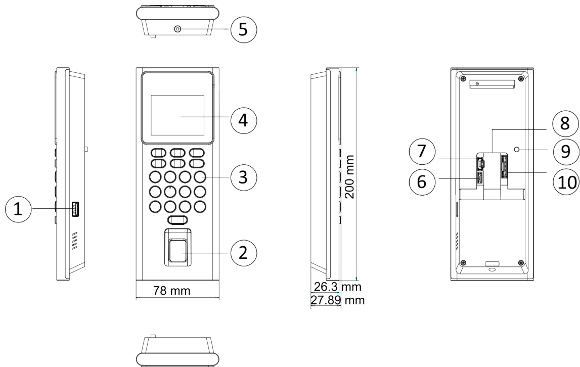
Figure 1-1 Appearance
