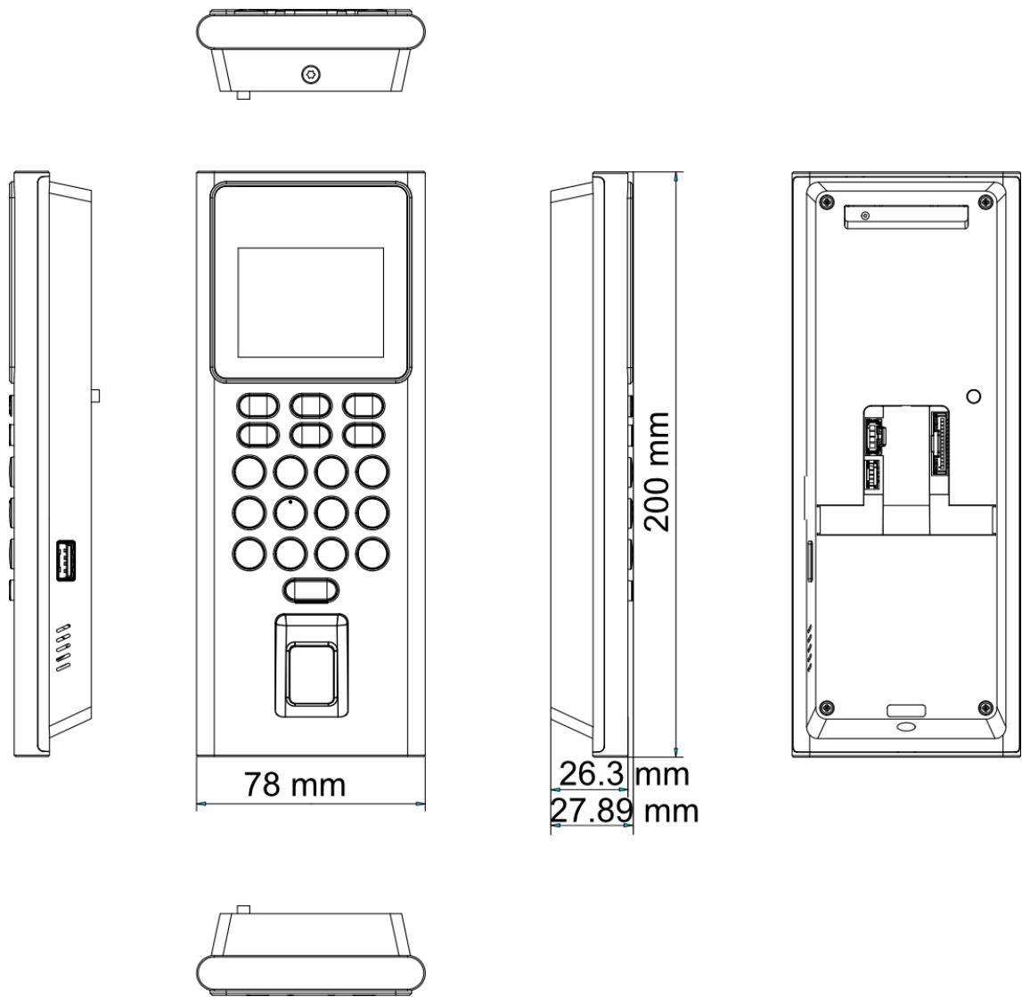
Figure B-1 Dimension
