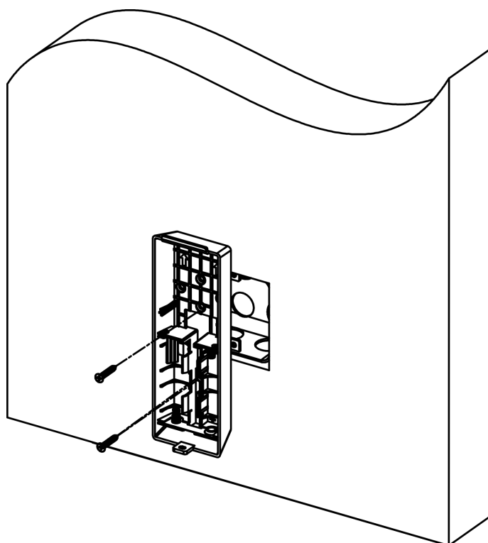
Figure 2-5 Install Mounting Plate
