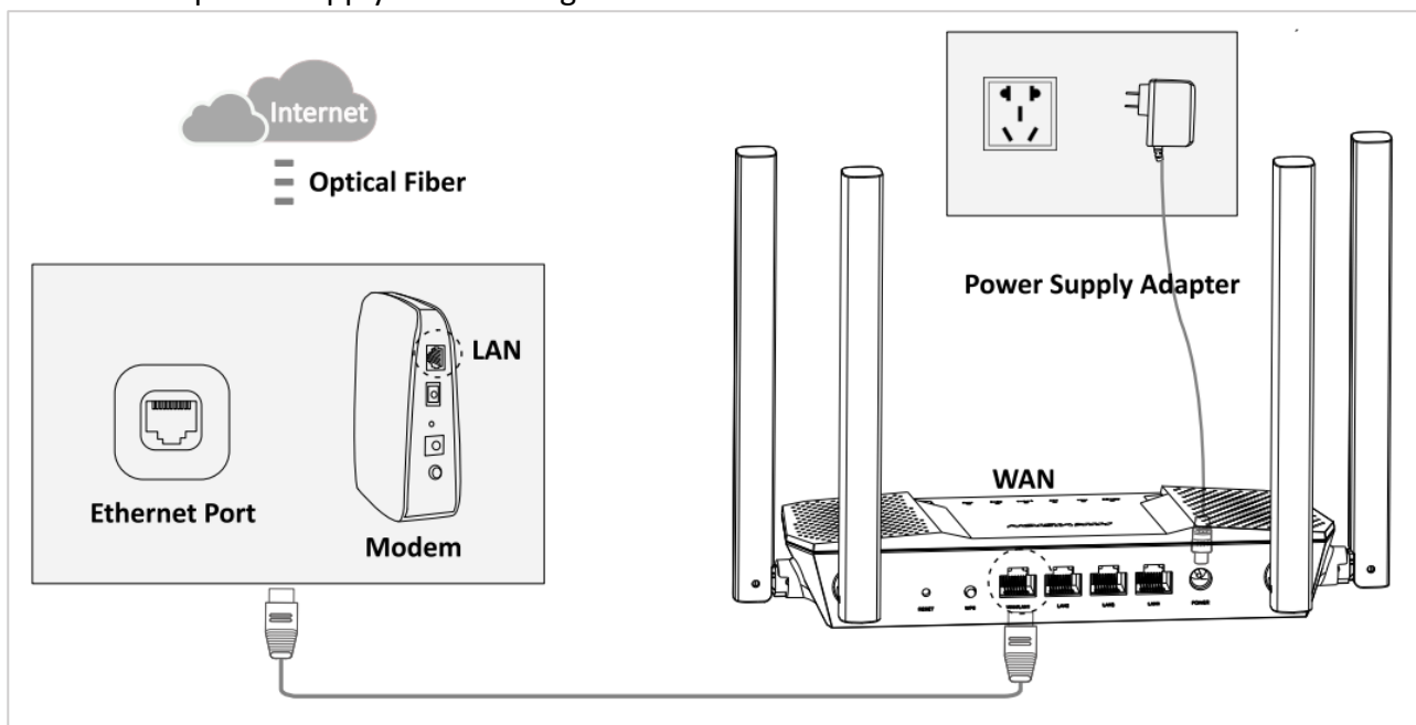
Figure 1-1 Wiring
