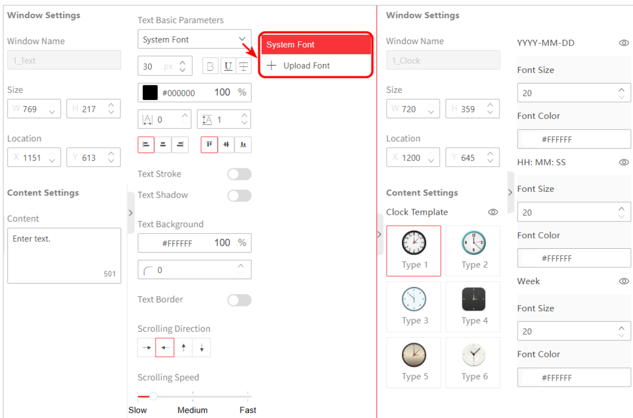
Figure 3-29 Configure Text/Clock
