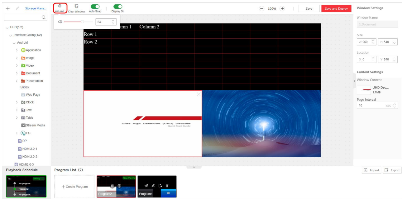
Figure 3-25 Manage Program
