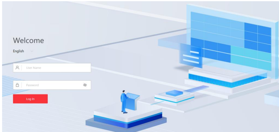
Figure 2-5 Login Page
