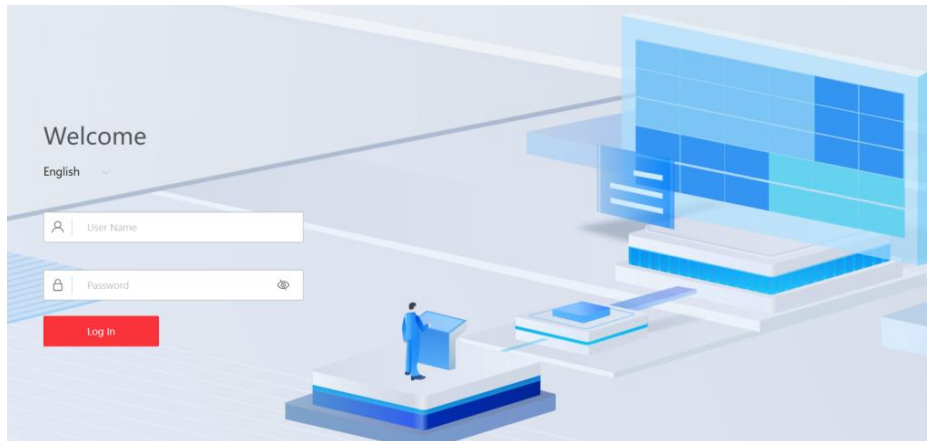
Figure 2-2 Login Page
