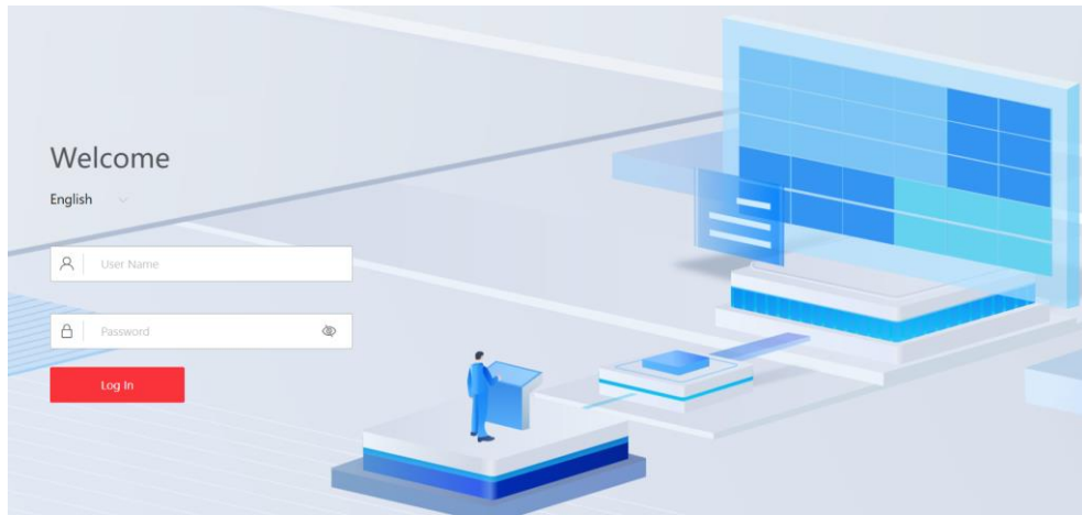
Figure 2-7 Login Page
